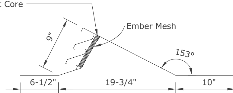
SECTION VIEW
