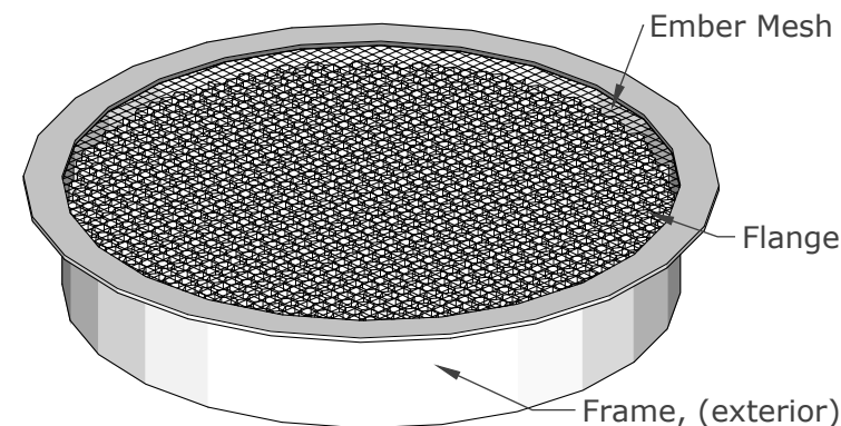
ISOMETRIC VIEW
