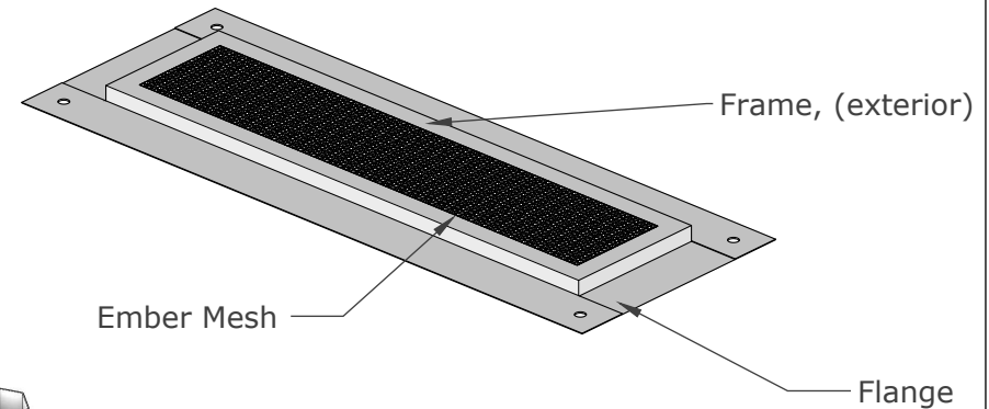
ISOMETRIC VIEW
