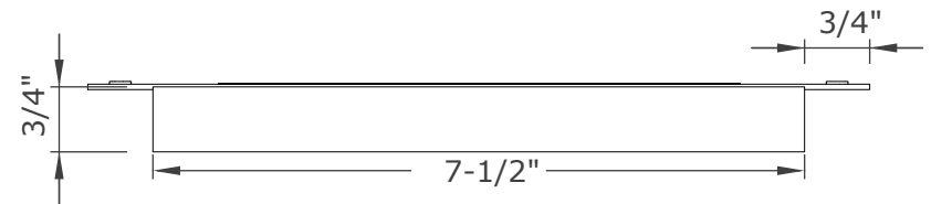
SIDE VIEW
