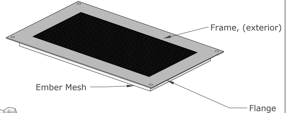
ISOMETRIC VIEW
