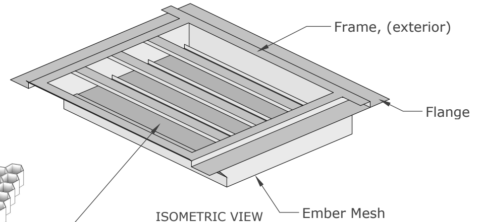
ISOMETRIC VIEW
