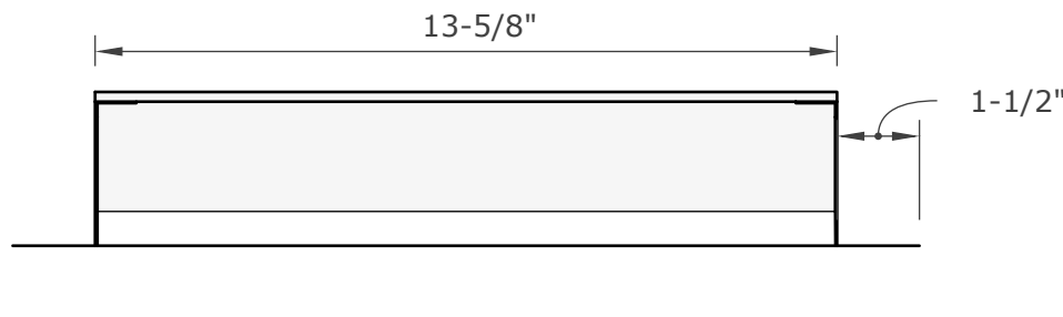
END VIEW
