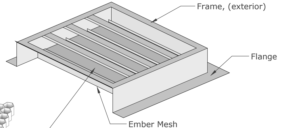
ISOMETRIC VIEW
