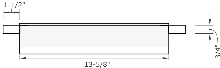
END VIEW
