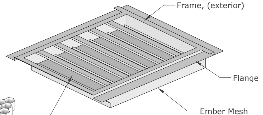
ISOMETRIC VIEW
