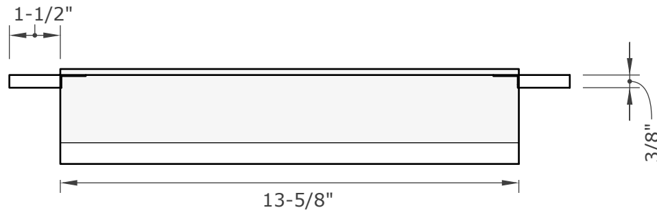
END VIEW
