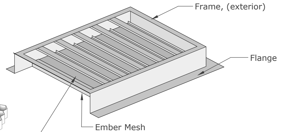
ISOMETRIC VIEW
