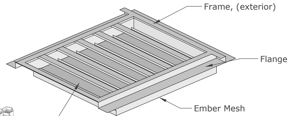
ISOMETRIC VIEW
