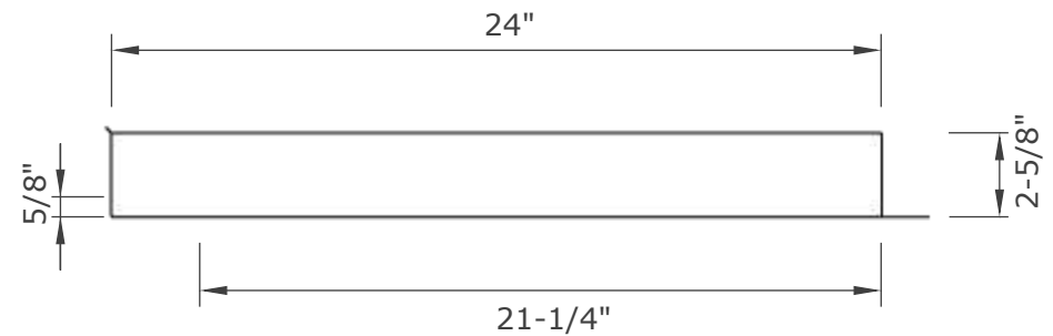
SIDE VIEW
