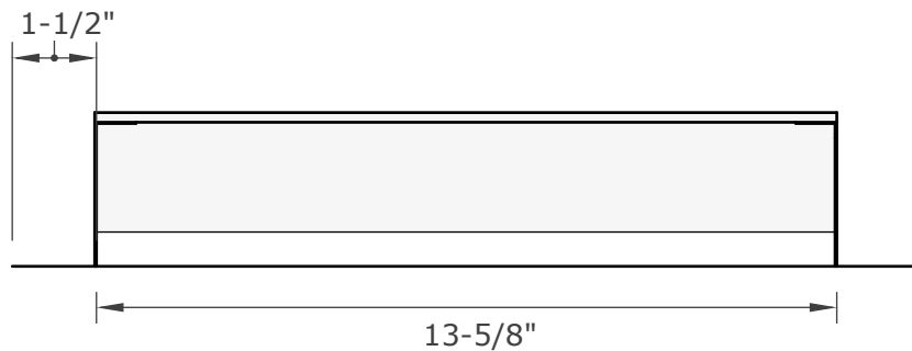
END VIEW
