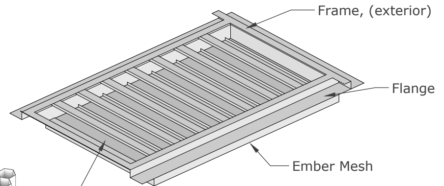
ISOMETRIC VIEW
