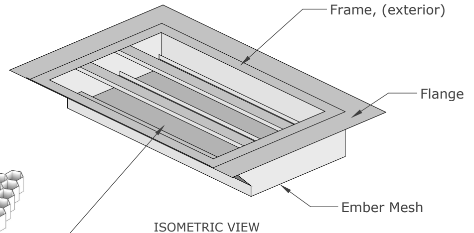
ISOMETRIC VIEW
