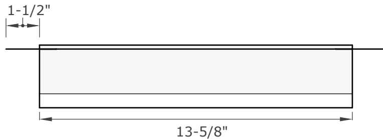
END VIEW
