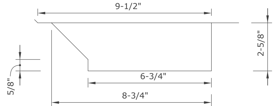
END VIEW
