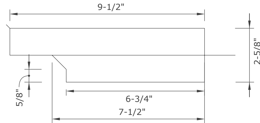
END VIEW
