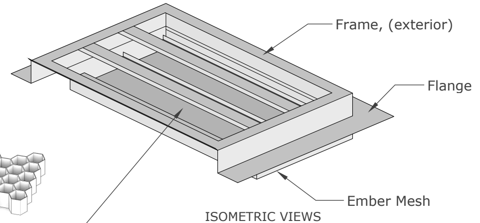
Intumescent Core
