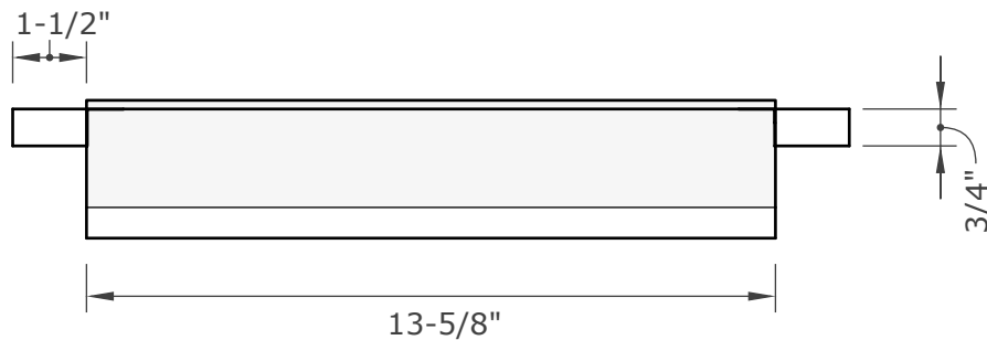
END VIEW
