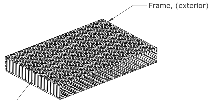
ISOMETRIC VIEWS
