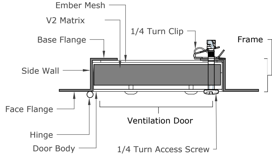
DETAILED VIEW
