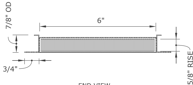
END VIEW
