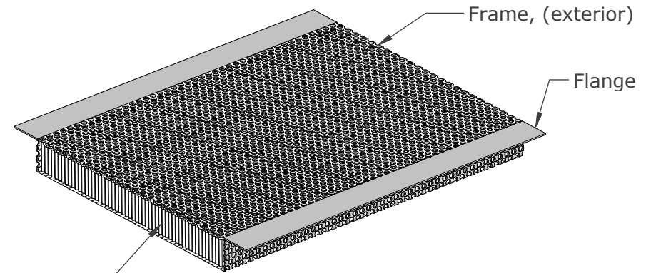
ISOMETRIC VIEWS
